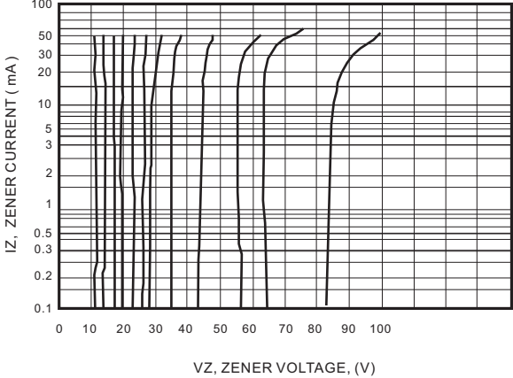
Fig.6 VZ = 12 Thru 82 Volts
