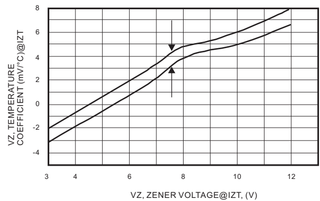
Fig 4. Units To 12 Volts
