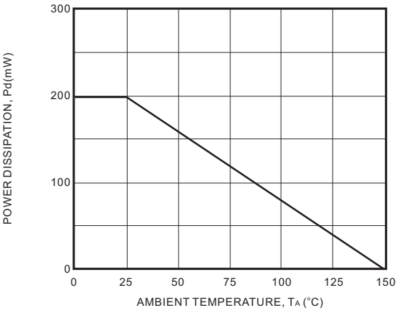
FIG. 2-DRATING CURVE
