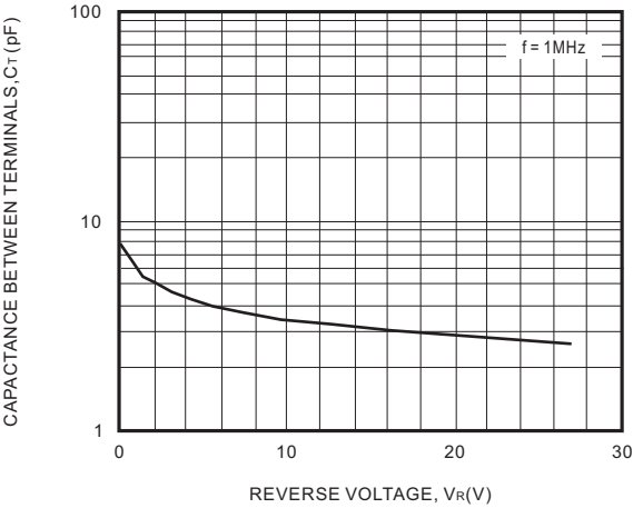
FIG. 4-VR-CT CHARACTERISTICS
