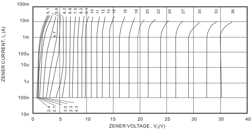
FIG.1-ZENER VOLTAGE CHARACTERISTICS
