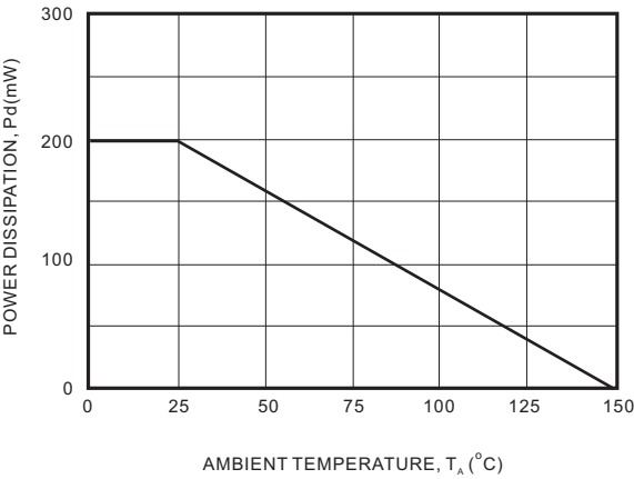
FIG. 2-DRATING CURVE
