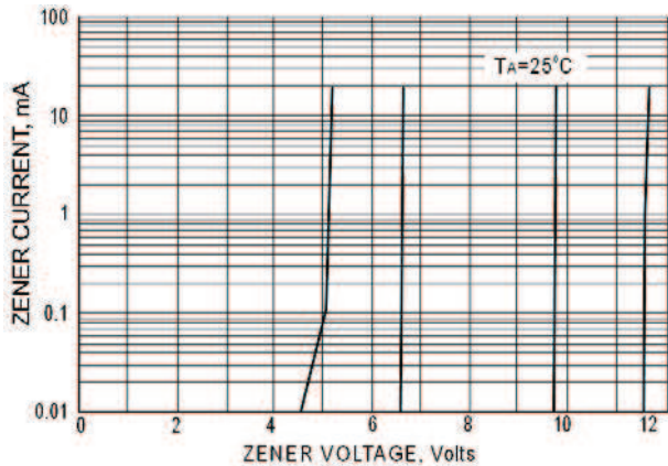
FIG. 5-ZENER BREAKDOWN CHARACTERISTICS
