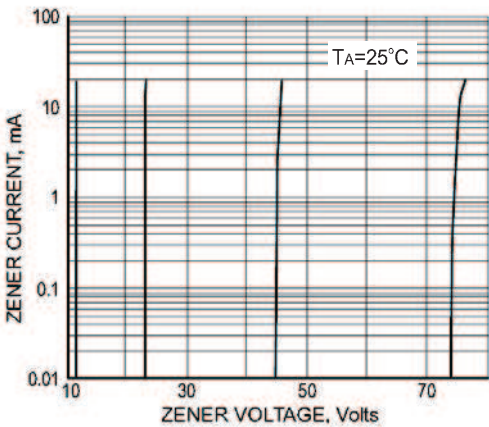
FIG. 6-ZENER BREAKDOWN CHARACTERISTICS
