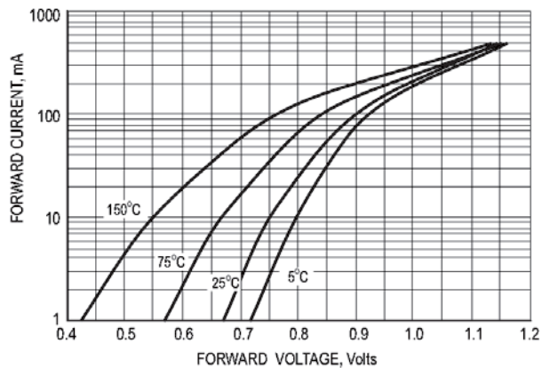
FIG. 3-TYPICAL FORWARD VOLTAGE
