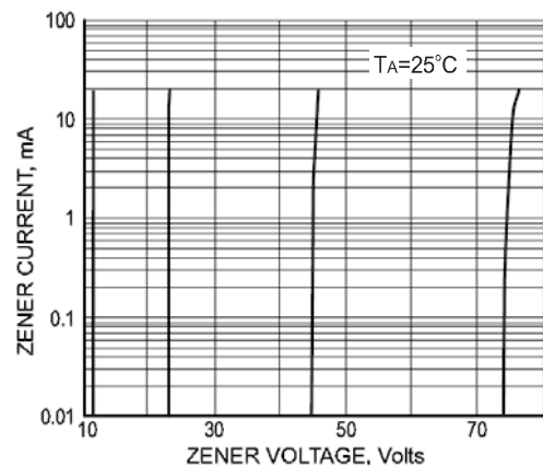
FIG. 6-ZENER BREAKDOWN CHARACTERISTICS
