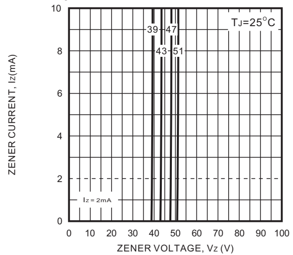
Fig.16 ZENER VOLTAGE CHARACTERISTICS
