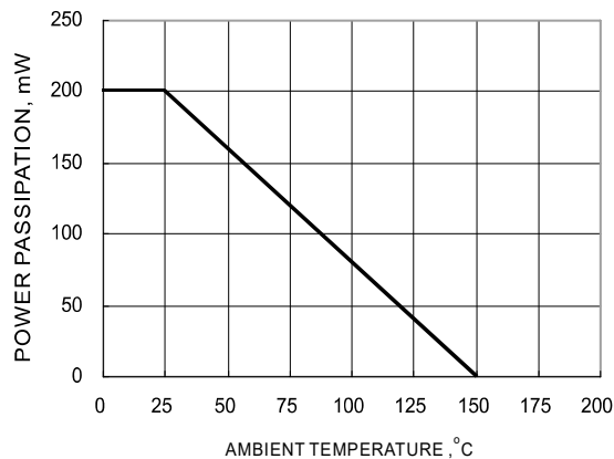
FIG. 1-POWER DISSIPATION VS. AMBIENT TEMP.
