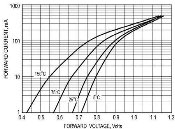
FIG. 3-TYPICAL FORWARD VOLTAGE
