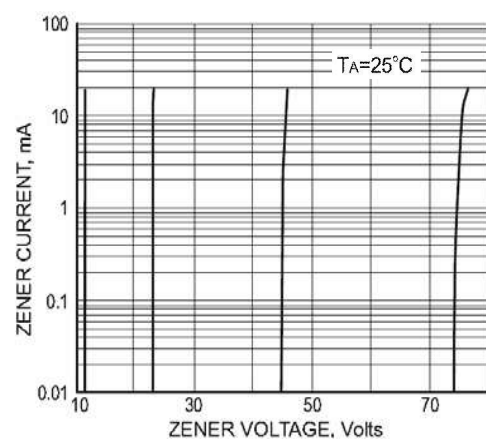
FIG. 6-ZENER BREAKDOWN CHARACTERISTICS
