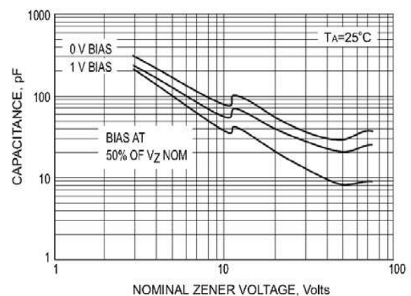
FIG. 4-TYPICAL CAPACITANCE
