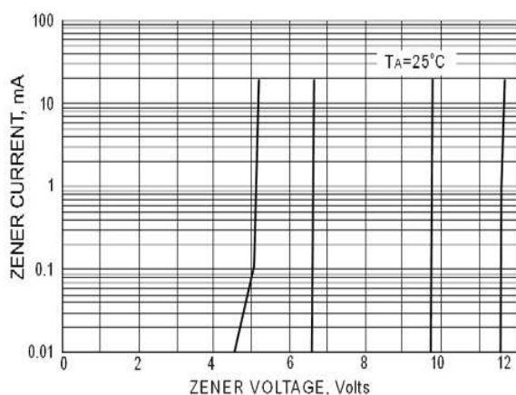
FIG. 5-ZENER BREAKDOWN CHARACTERISTICS
