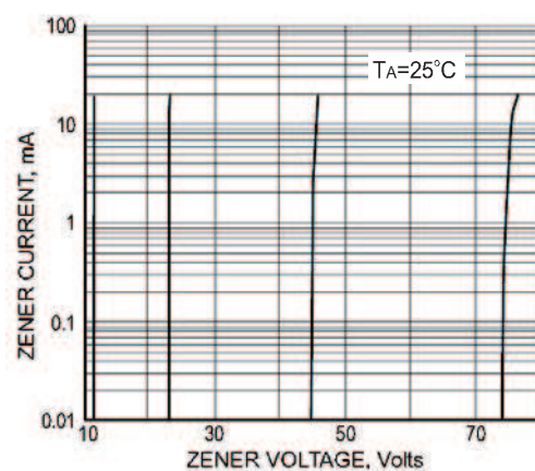
FIG. 6-ZENER BREAKDOWN CHARACTERISTICS
