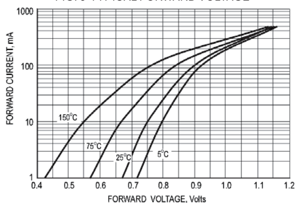
FIG. 3-TYPICAL FORWARD VOLTAGE
