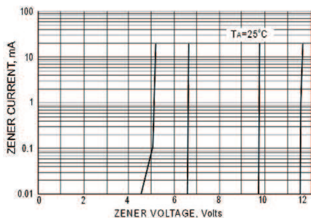
FIG. 5-ZENER BREAKDOWN CHARACTERISTICS
