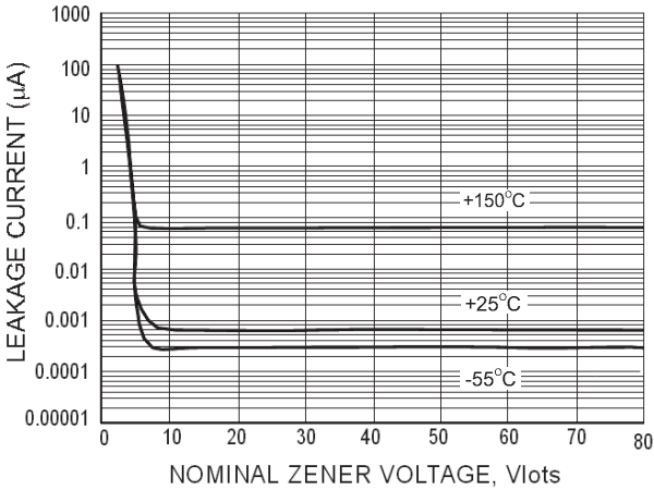
FIG. 7-TYPICAL LEAKGE CURRENT
