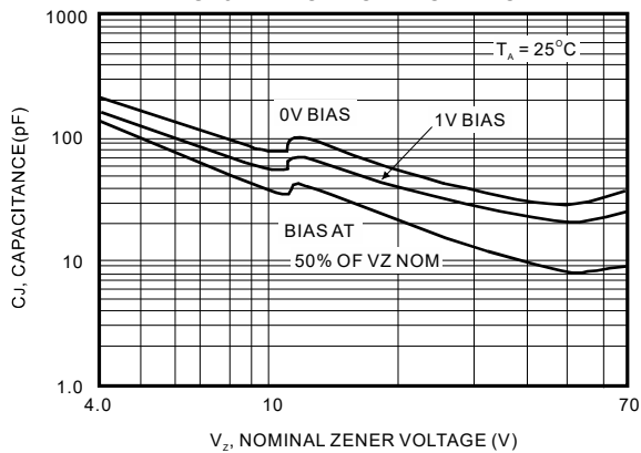
FIG. 3-TYPICAL CAPACITANCE
