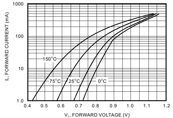
FIG. 2-TYPICAL FORWARD VOLTAGE
