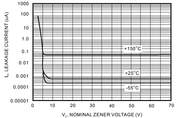
FIG. 4-TYPICAL LEAKAGE CURRENT
