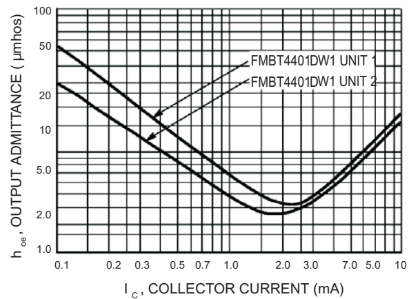
Figure 14. Output Admittance
