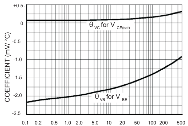
Figure 18. Temperature Coefficients
