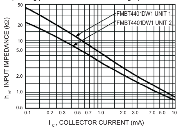
Figure 12. Input Impedance
