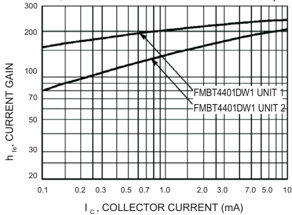
Figure 11. Current Gain
