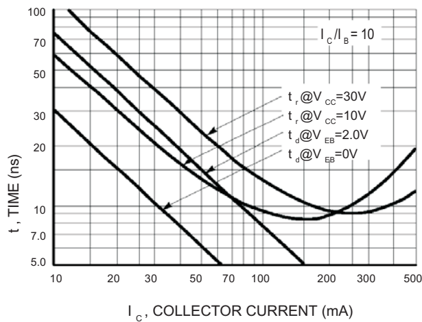
Figure 5. Turn-On Time
