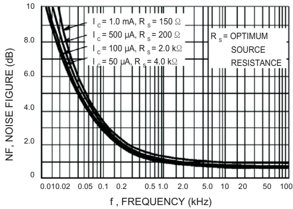
Figure 9. Frequency Effects
