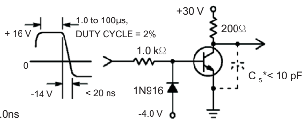
Figure 2. Turn-Off Time
