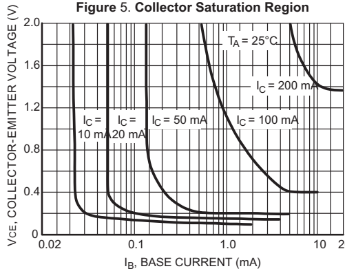
Figure 5. Collector Saturation Region
