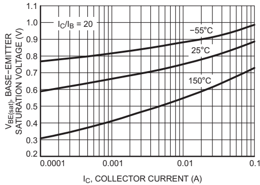
Figure 19. Base Emitter Saturation Voltage vs. Collector Current
