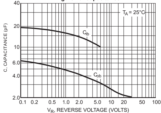
Figure 15. Capacitance
