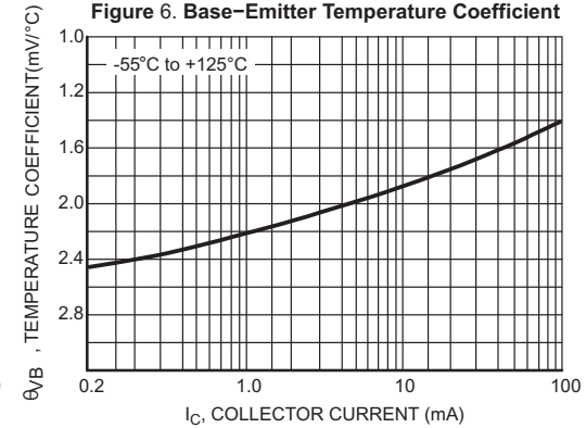
Figure 6. Base-Emitter Temperature Coefficient
