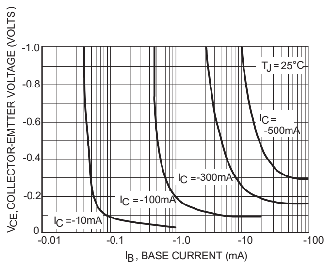
Figure 5. Saturation Region
