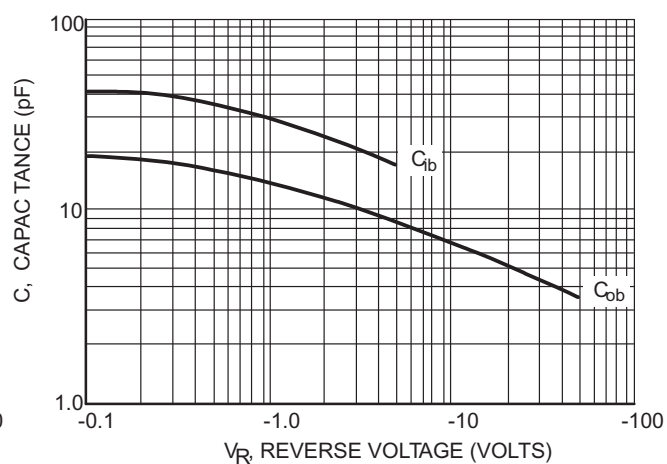
Figure 23. Capacitances
