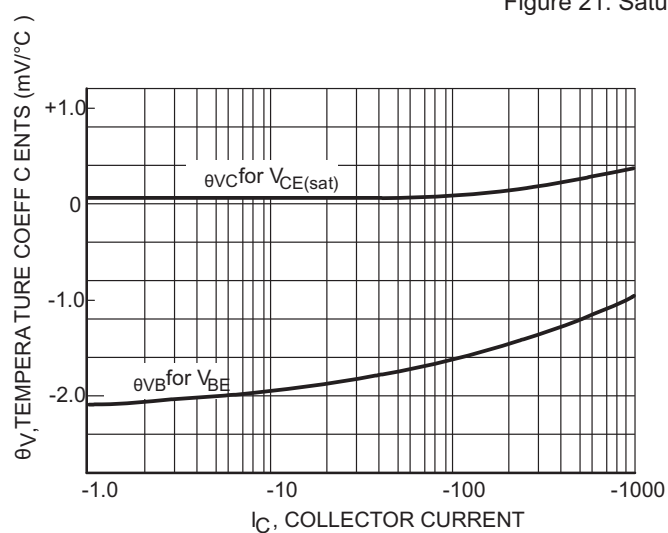
Figure 22. Temperature Coefficients
