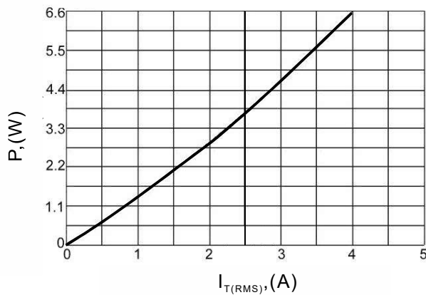
Maximum power dissipation vs. On-state current
