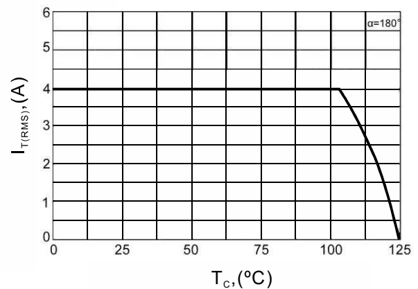
On-state current vs. Case temperature
