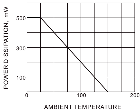
Fig.4 DERATING CURVE
