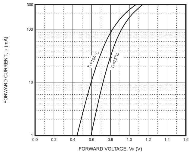
Fig.1- Forward Characteristics
