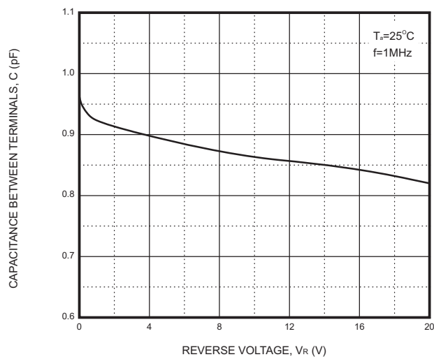
Fig.3- Capacitance Characteristics
