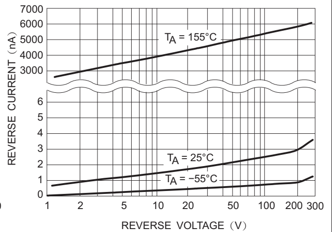
Figure 2. Reverse Leakage
