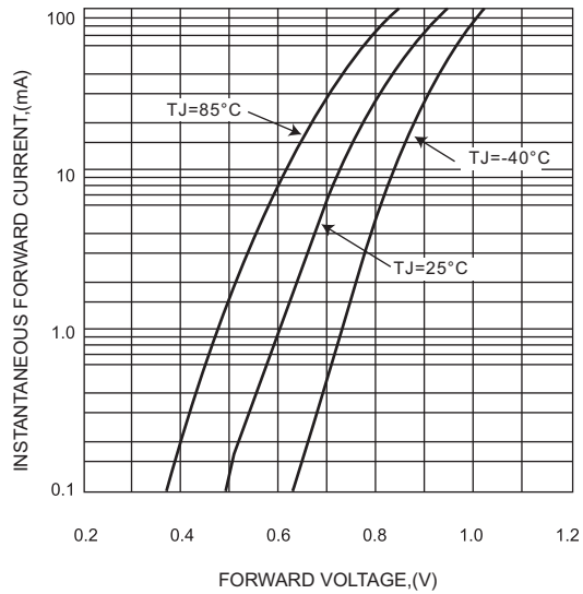
FIG.1-TYPICAL FORWARD CHARACTERISTICS
