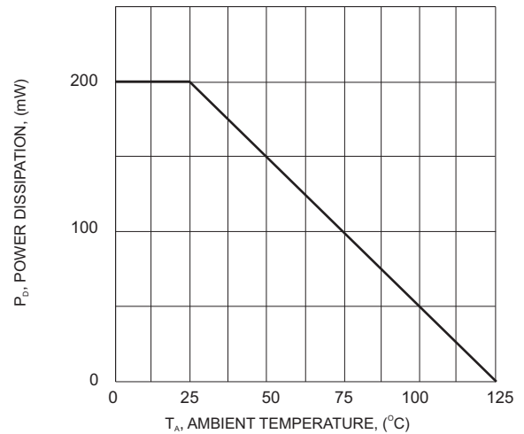
FIG.4 - TYPICAL POWER DERATING CURVE
