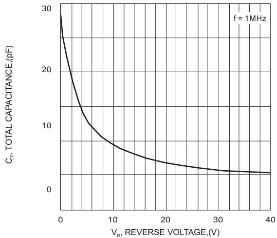
FIG.3-TYPICAL CAPACITANCE CAPACITANCE
