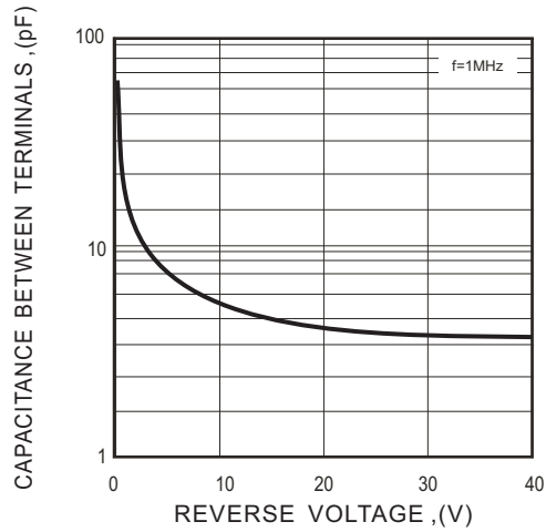
FIG.3-TYPICAL TERMINALS CAPACITANCE
