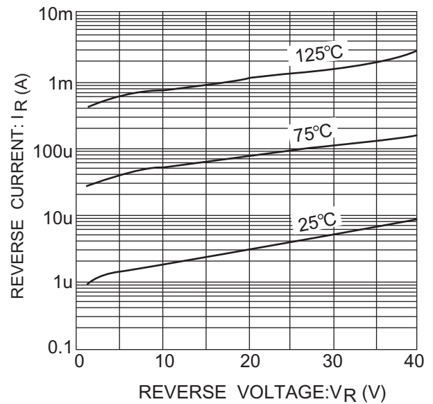
Fig.2 Reverse characteristics
