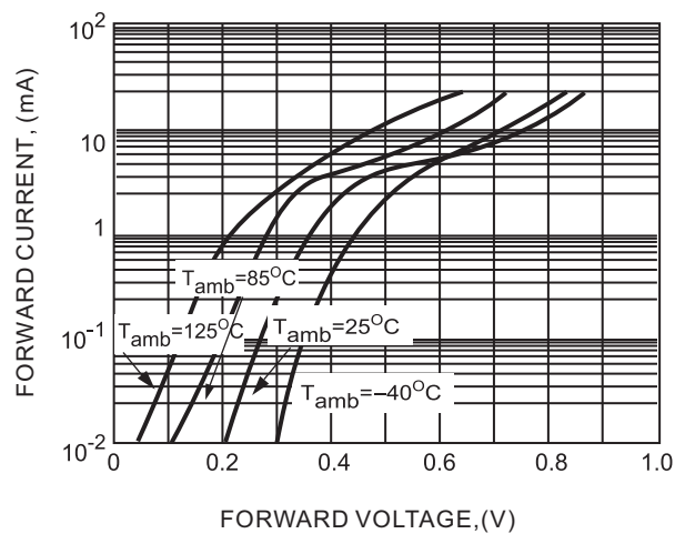
FIG.1-FORWARD CHARACTERISTICS
