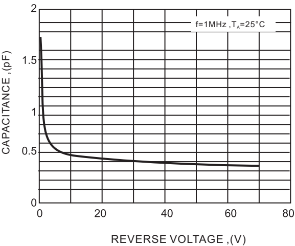
FIG.4-CAPACITANCE CHARACTERISTICS
