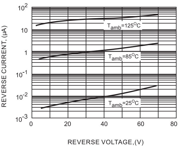
FIG.2-REVERSE CHARACTERISTICS
