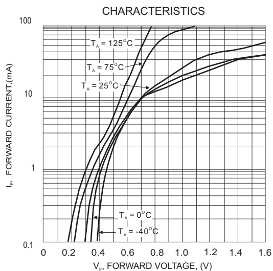
FIG.1-TYPICAL FORWARD
