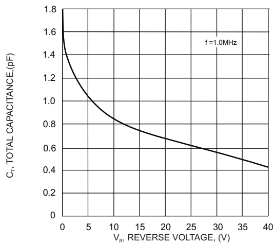
FIG.3-TYPICAL JUNCTION CAPACITANCE
