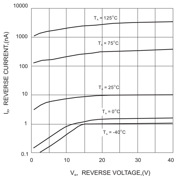
FIG.2-TYPICAL REVERSE CHARACTERISTICS
