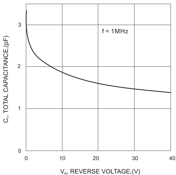
FIG.3-TYPICAL CAPACITANCE
