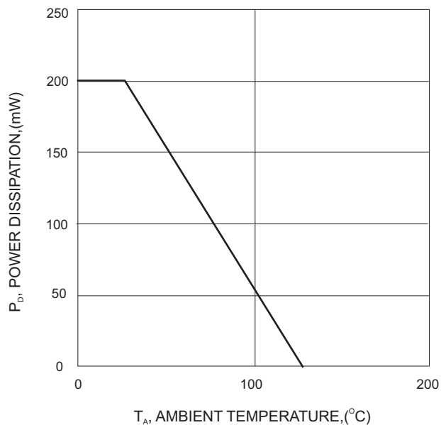
FIG.4-POWER DERATING CURVE
