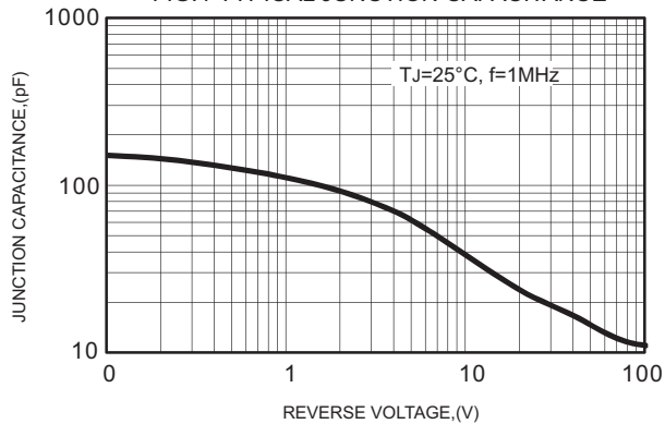
FIG.4-TYPICAL JUNCTION CAPACITANCE
