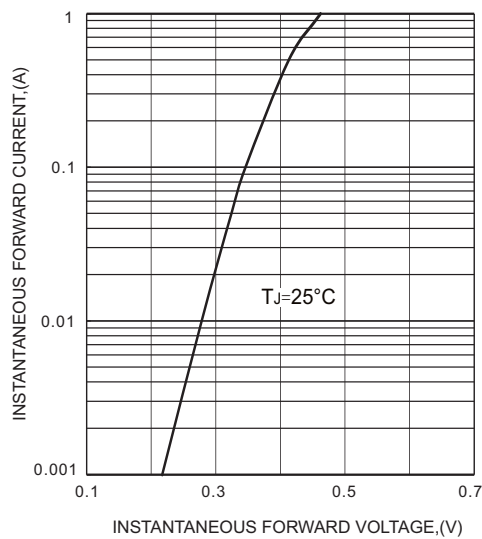
FIG.3-TYPICAL FORWARD CHARACTERISTICS
