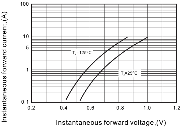
Typical instantaneous forward characteristics
