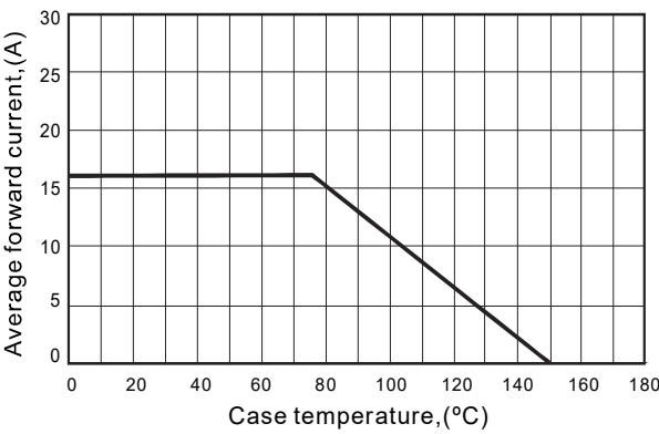
Typical forward current derating curve
