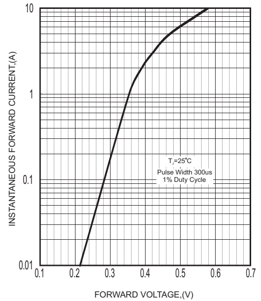
FIG.2-TYPICAL FORWARD CHARACTERISTICS
