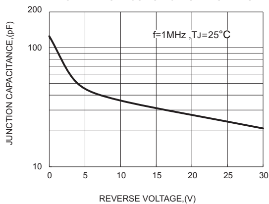
FIG.4-TYPICAL JUNCTION CAPACITANCE
