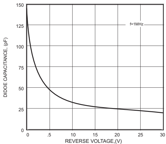
FIG.4-TYPICAL DIODE CAPACITANCE
