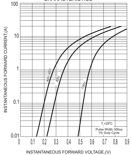
FIG.2-TYPICAL FORWARD CHARACTERISTICS
