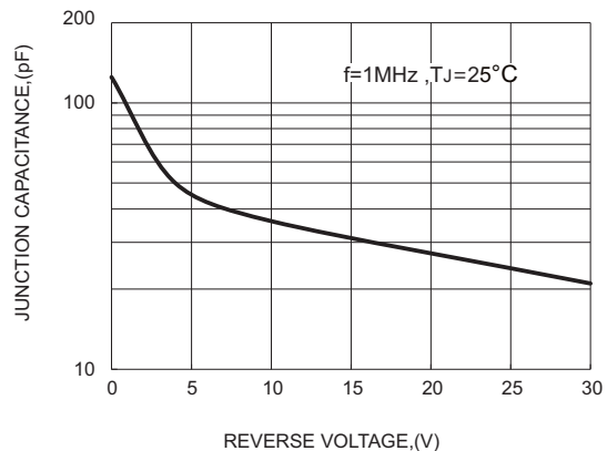
FIG.5-TYPICAL JUNCTION CAPACITANCE
