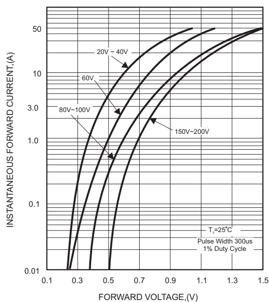
FIG.2-TYPICAL FORWARD CHARACTERISTICS
