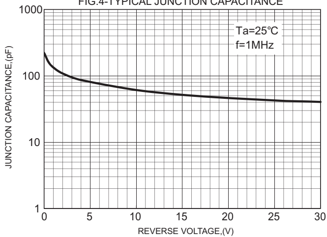
FIG.4-TYPICAL JUNCTION CAPACITANCE
