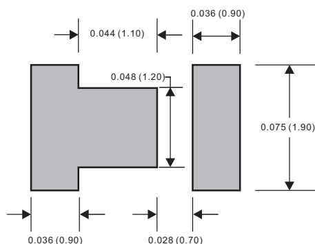
SOD-123HT
