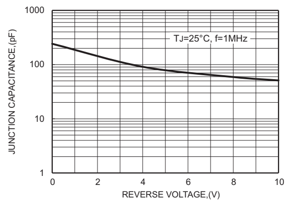
FIG.5-TYPICAL JUNCTION CAPACITANCE
