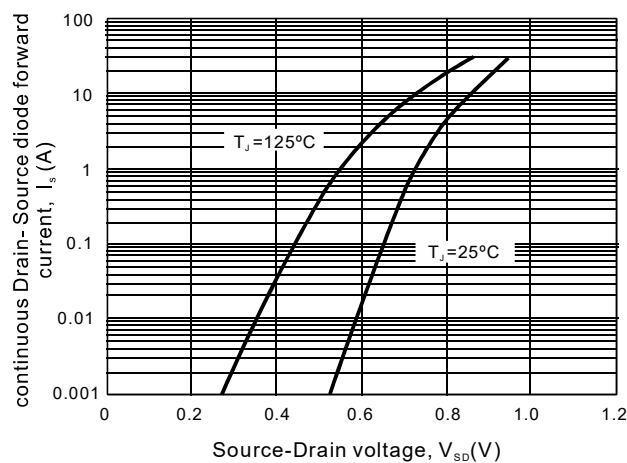
Body-diode characteristics
