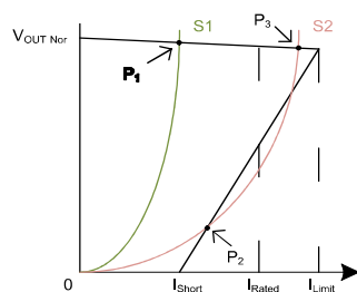
Figure 9-3. Nonlinear Load Example
