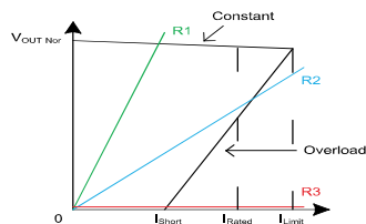
Figure 9-1. Fold-back Current Limit
