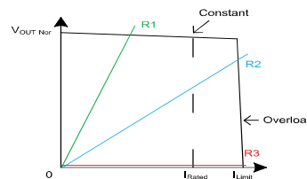
Figure 9-2. Brick-wall Current Limit
