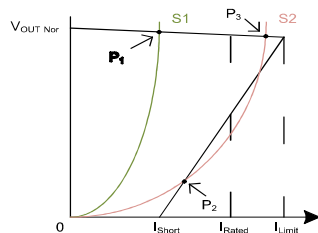
Figure 9-3. Nonlinear Load Example
