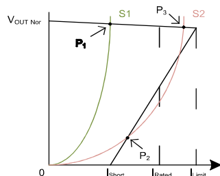
Figure 9-3. Nonlinear Load Example
