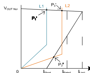
Figure 9-4. Active Load Profile
