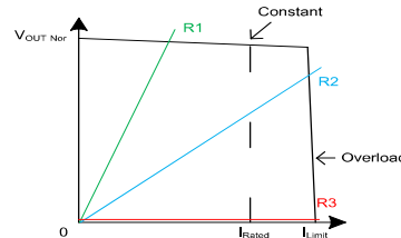
Figure 9-2. Brick-wall Current Limit
