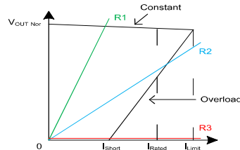
Figure 9-1. Fold-back Current Limit
