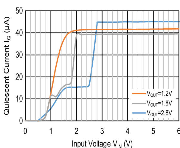
Quiescent Current
