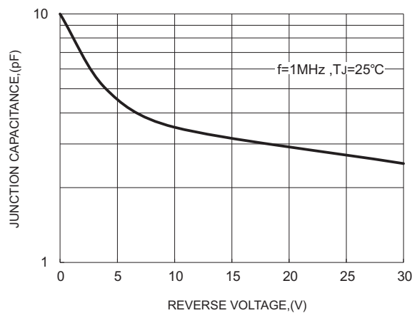
FIG.5-TYPICAL JUNCTION CAPACITANCE
