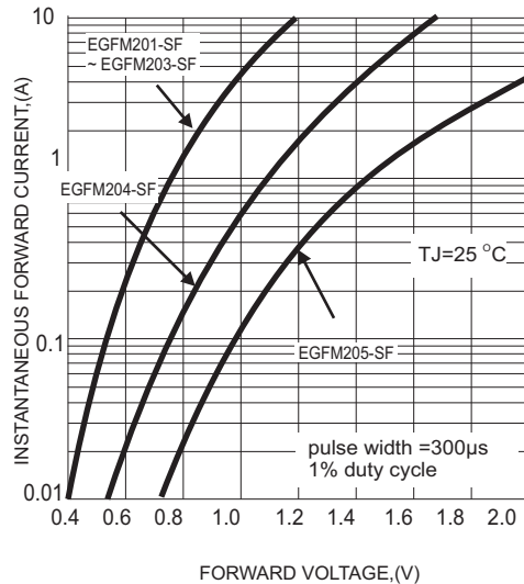
FIG.1-TYPICAL FORWARD CHARACTERISTICS
