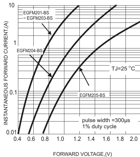
FIG.1-TYPICAL FORWARD CHARACTERISTICS
