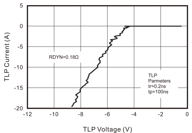
FIG.6 TLP Negative I-V Curve
