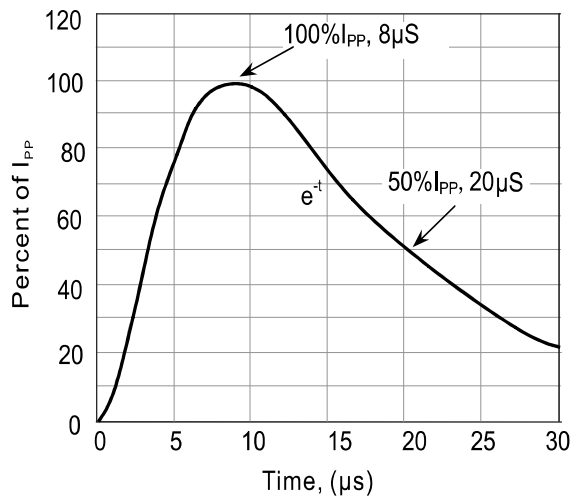
Pulse waveform, 8/20 \mu s
