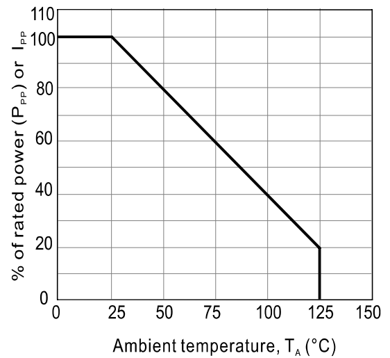
Pulse derating curve
