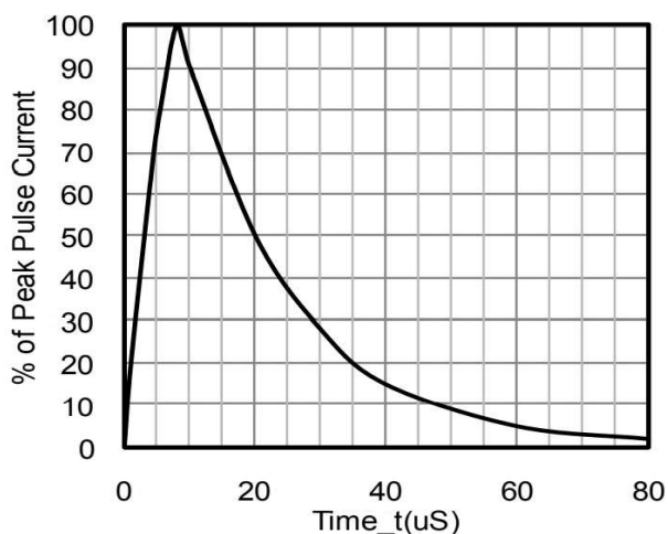
8 X 20 \mu s Pulse Waveform
