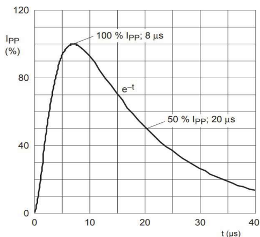
8/20 \mu s pulse waveform according to IEC 61000-4-5
