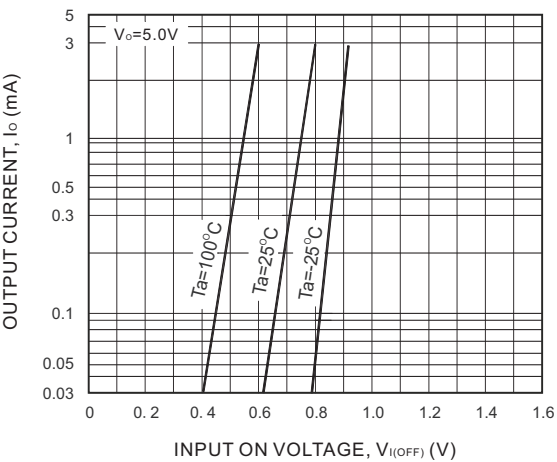
I_o - V_{I(OFF)}
