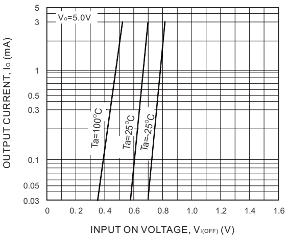
I_o - V_{I(OFF)}
