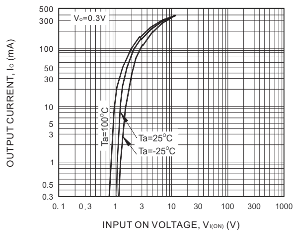
I_o - V_{I(ON)}
